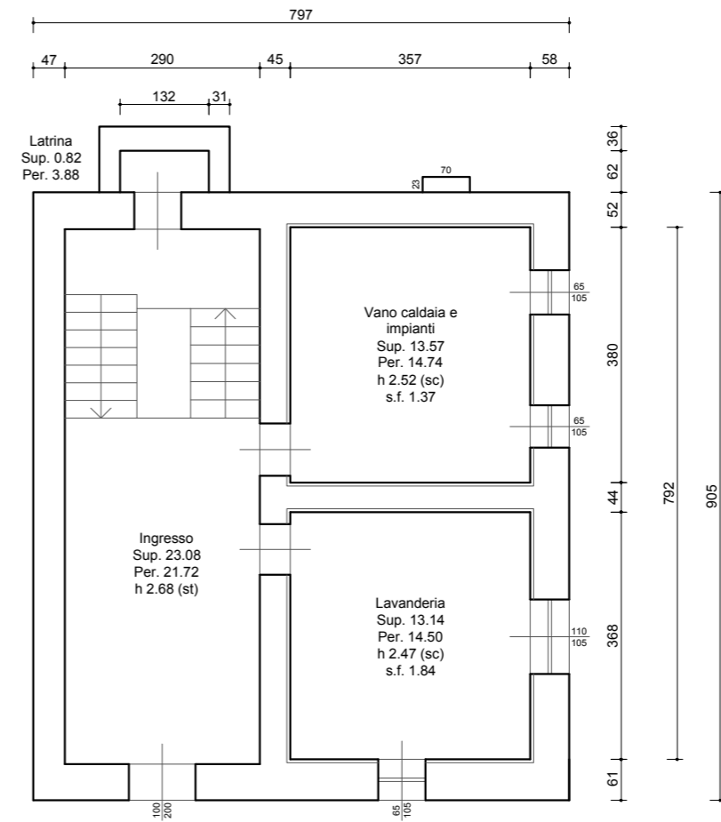
Piano terra Scala 1/100
